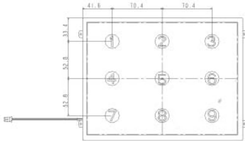
Fig8-1 Measuring point
