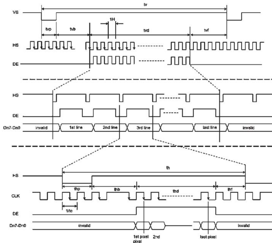
Figure 11.1 Input timing
